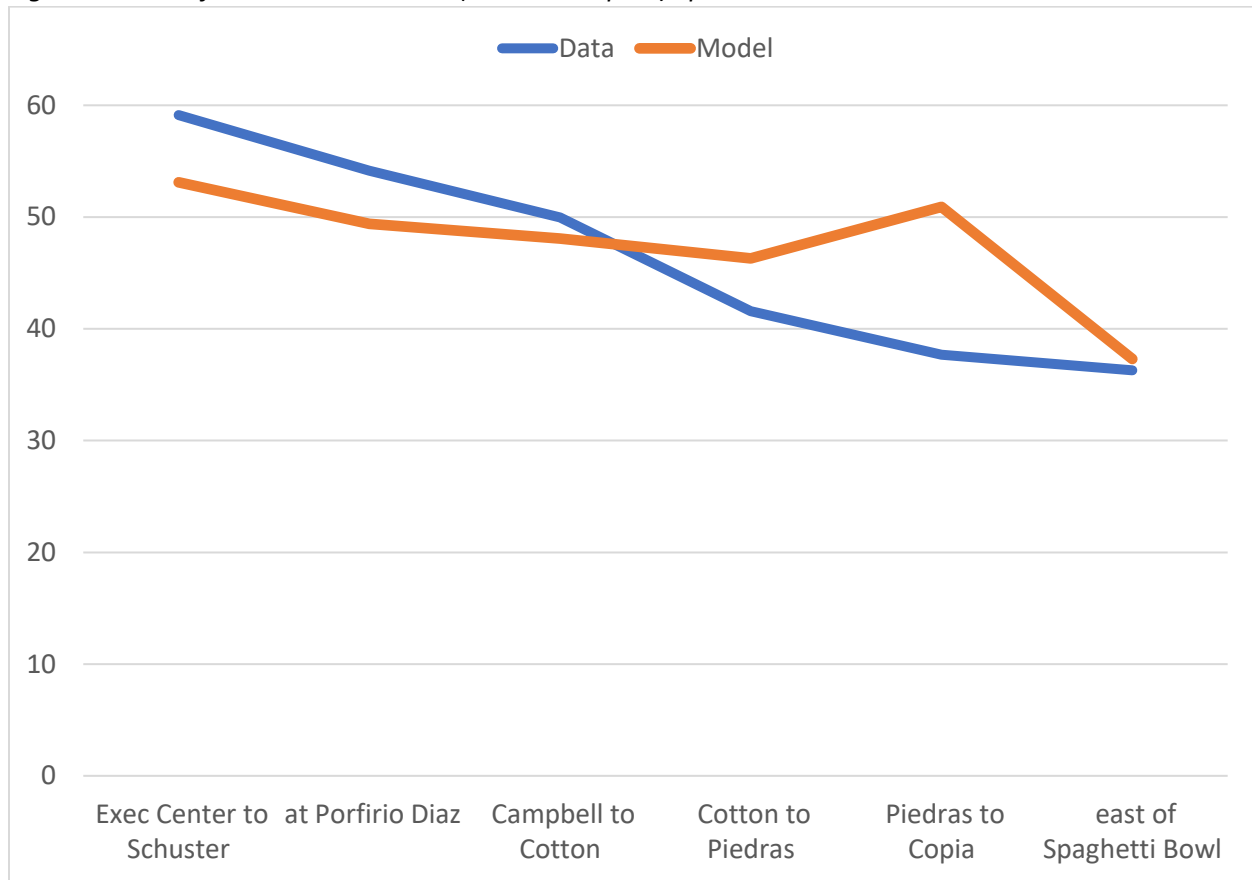
Figure 7: 2019 Afternoon Peak Period (2:30 – 6:30 p.m.) Speed vs. 2017 Base Year Model
