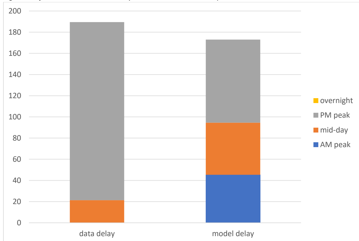
Figure 9: Afternoon Peak Period Delay Eastbound Piedras to Copia – Data vs. Model
