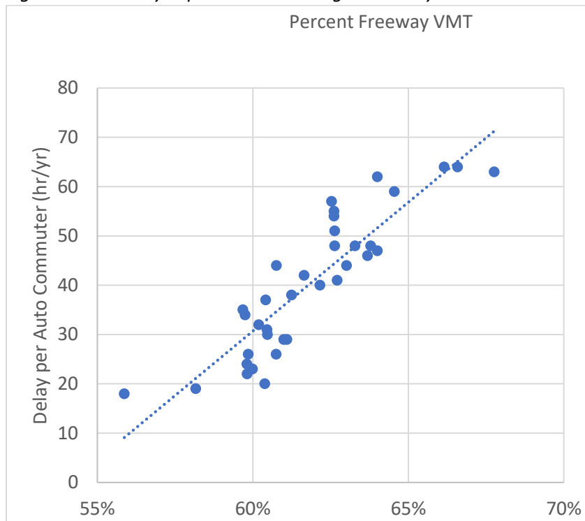
Figure 12: Freeway Expanses Causes Regional Delay
