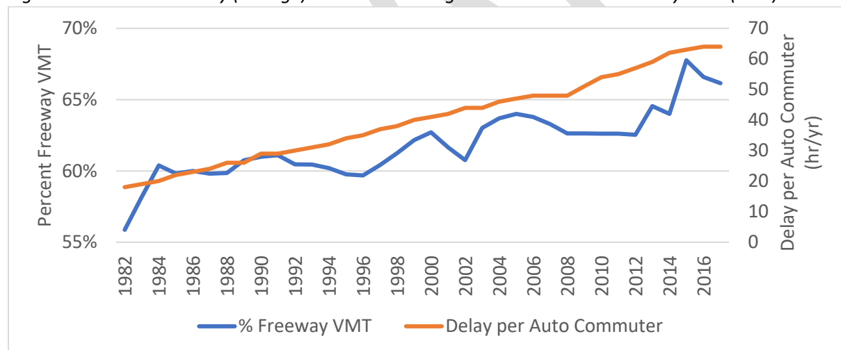
Figure 11: Growth in Delay (Orange) Has Grown Along with Growth in % Freeway VMT (Blue)
