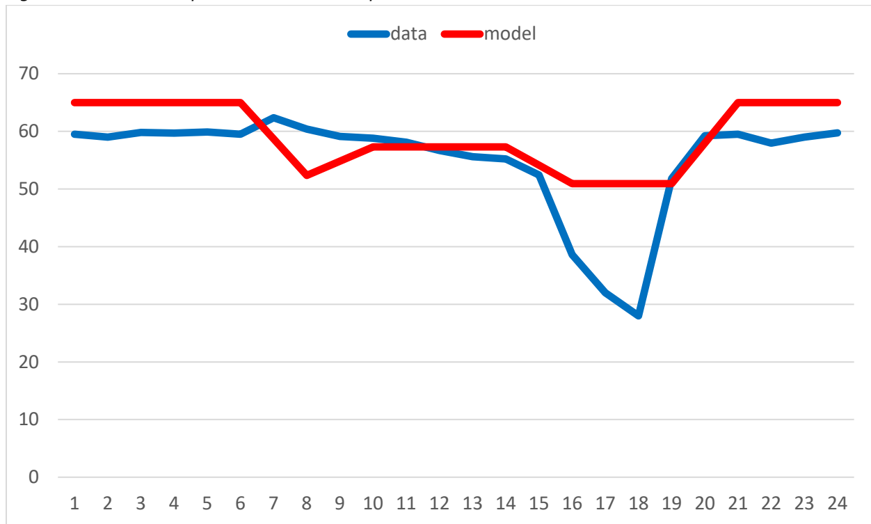
Figure 8: Piedras to Copia Eastbound 2019 Speed vs. 2017 Base Year Model
