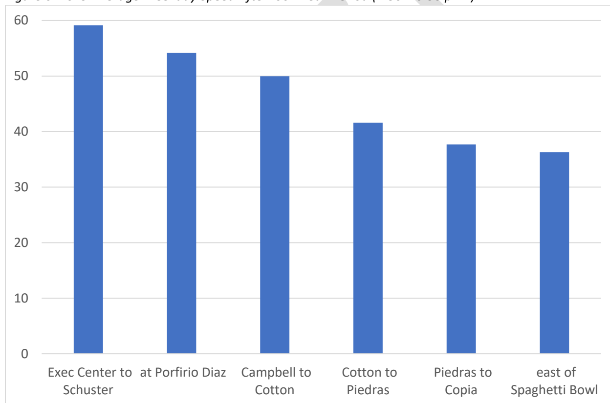
Figure 6: 2019 Average Weekday Speed Afternoon Peak Period (2:30 – 6:30 p.m.)
